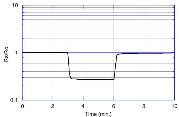
Fig. 10 - Gas response to EtOH
