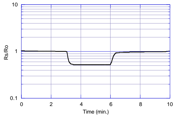
Fig. 11 - Gas response to ammonia
